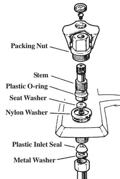
Common Faucet Assembly
